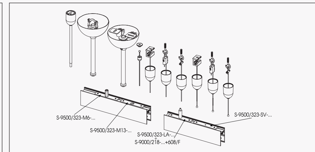
Accessories for „in row“ use junctions
